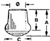
Art.PSP Piede scala a pera in pvc ø 35-38-40
